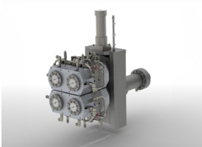
DOUBLE-HEAD DIE CHANGER WITH GAP ADJUSTMENT
